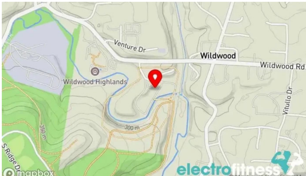
Raw training map
